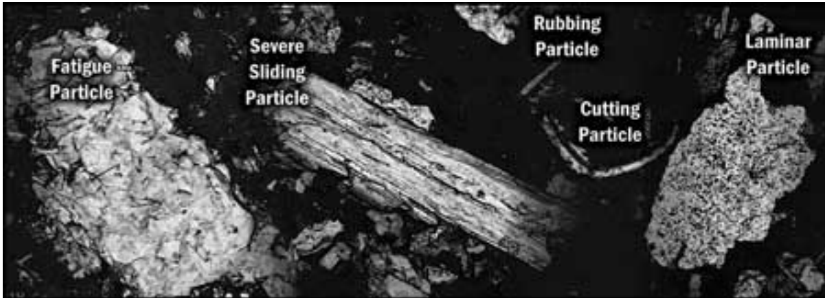
Wear particles generated from component failure.
